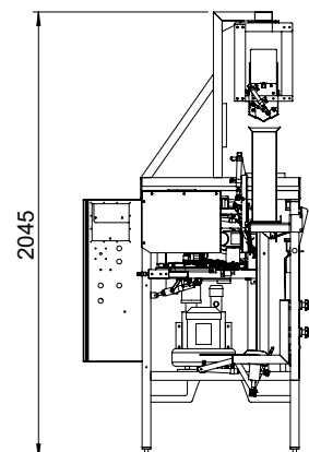
Example of carrot model PEB40G
