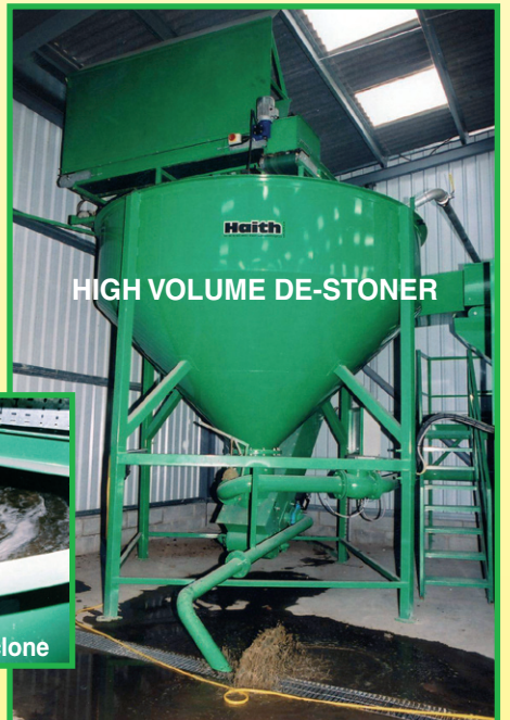
Stone removal on POTATOES
